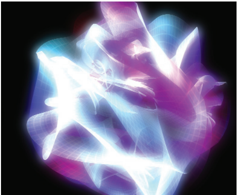
Calabi-Yau shapes, such as the one in this computer model, are theorized to possibly contain string theory’s added dimensions.
